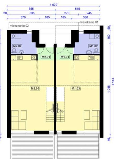
PARTER
